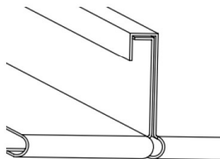
Hem Panel
