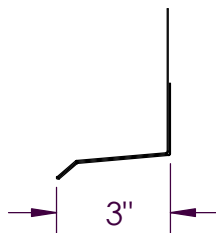
BASE TRIM / WINDOW HEAD TRIM
