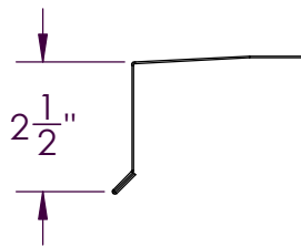
SILL TRIM
